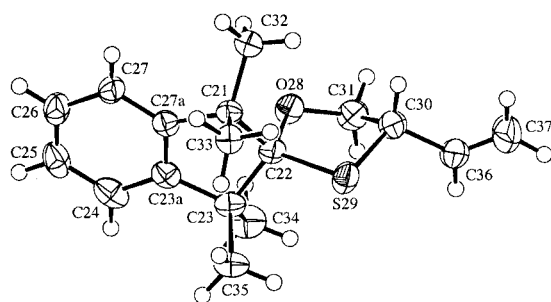
Figure 2. ORTEP plot [35] of the molecular structure of one of the two symmetry-independent molecules of ( S )- 12 (arbitrary numbering of the atoms; displacement ellipsoids with 50% probability).
