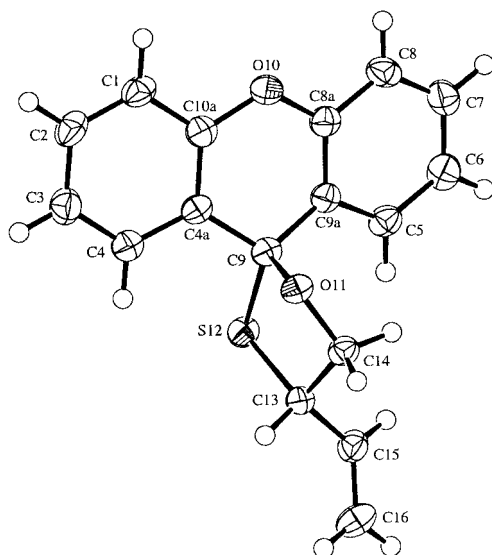
Figure 1. ORTEP plot [35] of the molecular structure of ( S )- 9 (arbitrary numbering of the atoms; displacement ellipsoids with 50% probability).
